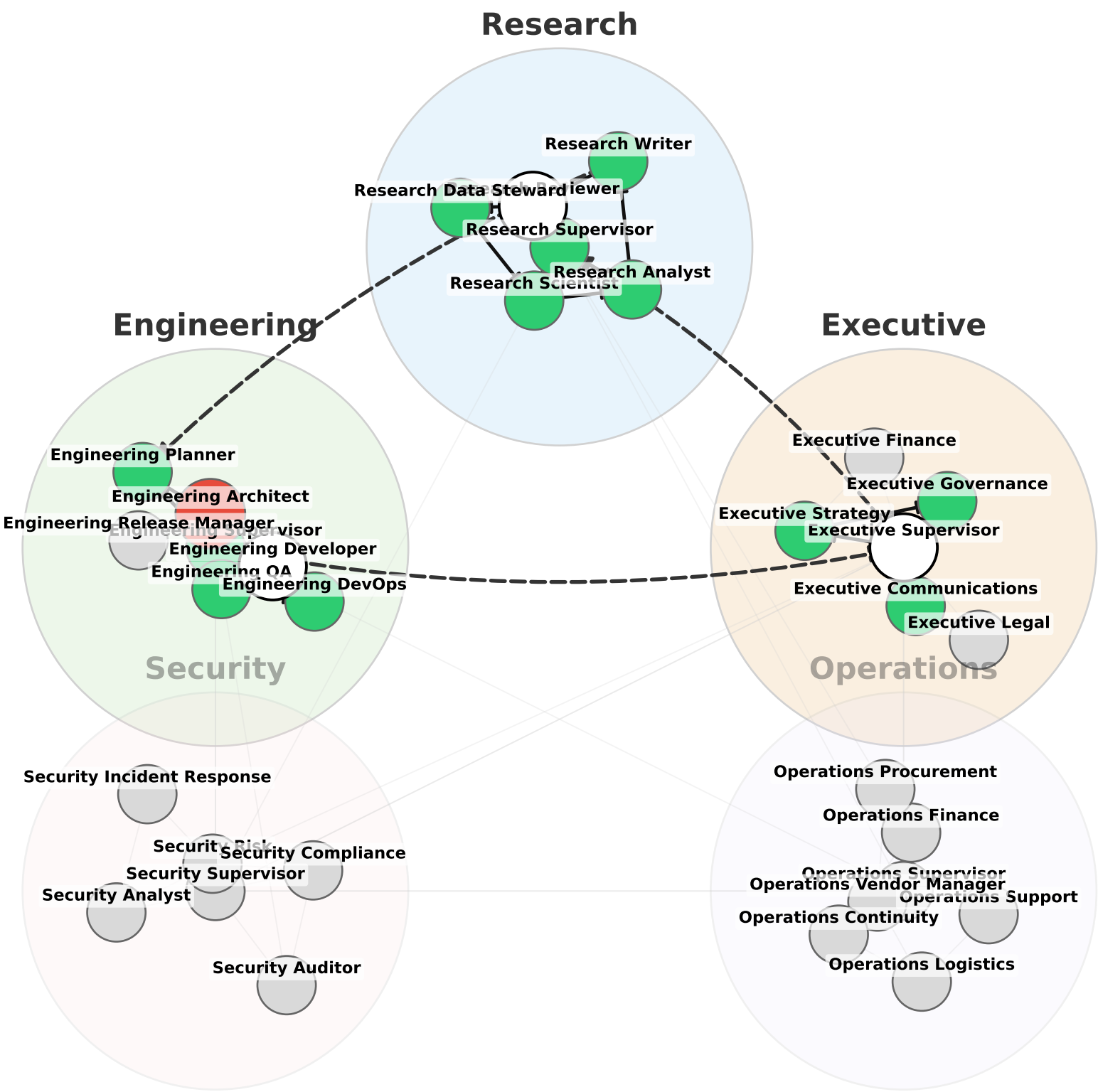
(a) Runtime Trust Graph
